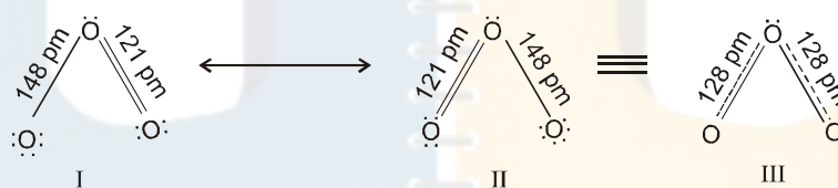
Resonance in the \text{O}_3 molecule
