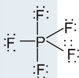
PF 5
