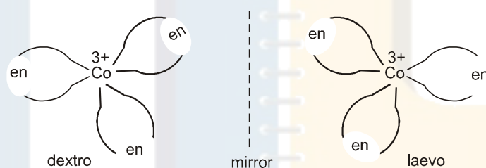
d and l of [\text{Co}(\text{en})_3]^{3+}
