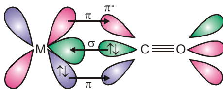
Synergic bonding
